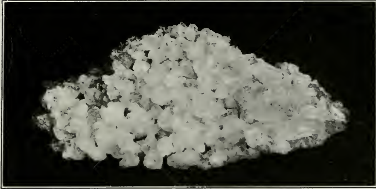
Fig. 2. Crystals of Thiosulphate of Soda or "Hypo".
